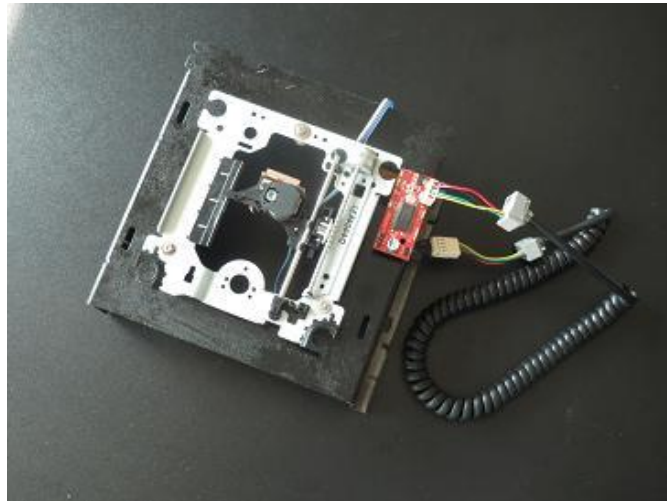
X axis + flexible wire + motor driver
