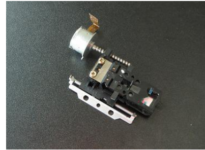
Y axis assemble sample Full step 0.18mm/p PARTS No,MS10015 / PARTS No,SY00-1 / PARTS No,SY00 / PARTS No,SY01 Price 11 Rm / pcs
