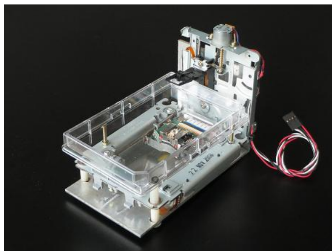
XYZ axis assemble sample
