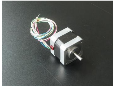
ORIENTAL STEP MOTOR PK244-02A 2PHASE 24V PARTS No,MS244 Price 55 Rm / pcs
