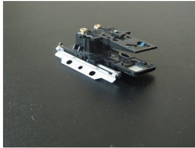
Y axis assemble sample Full step 0.18mm/p PARTS No,MS10015 / PARTS No,SY00-1 / PARTS No,SY00 / PARTS No,SY01 Price 11 Rm / pcs
