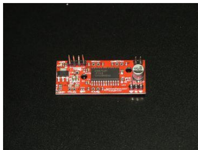
New STMicro technology ARM CoreM072P New EasyDriver ( 32bit RISC MCU DISCOVER ) PARTS No,ES072 Price 7 Rm / pcs
